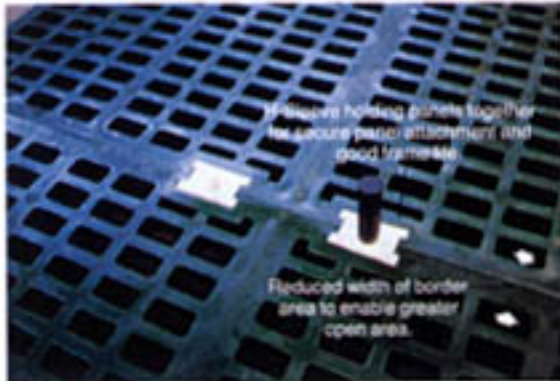
Replaceable huckbolted runner frame
